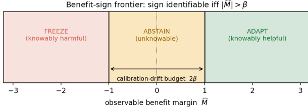
Fig. 2. The benefit-sign frontier. The sign of the adaptation benefit is identifiable from label-free evidence iff the population margin |M| exceeds the calibration-drift budget \beta . Outside the band KGA ADAPTS (knowably helpful) or FREEZES (knowably harmful); inside the band (the unknowable region), abstention is information-theoretically forced. (This is the population identifiability frontier of Theorem 2; the deployed finite-sample rule instead thresholds \hat{\Delta} \pm \varepsilon , Fig. 3.)
