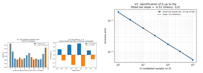
Fig. 9. One-bit identification (Synthetic validator; Thm. 5(ii)).
