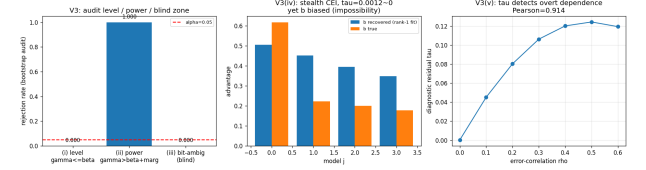
Fig. 10. Budget audit (Synthetic validator; Thm. 5(iv)).
