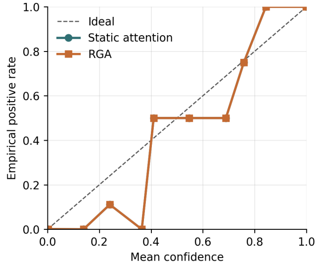
Fig. 13. Reliability diagram for static attention and RGA.
