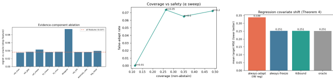
Fig. 5. Left: evidence-component ablation (disagreement dominates). Middle: \alpha sweep—safety vs coverage. Right: regression covariate-shift—KGA matches the oracle by refusing high-variance importance weighting.
