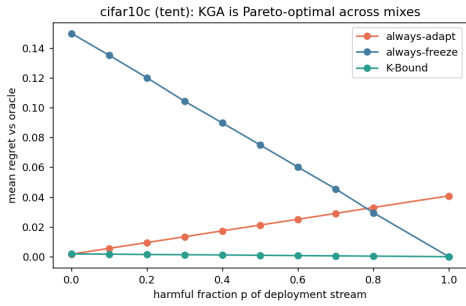
Fig. 3. CIFAR-10-C stress grid: regret-to-oracle vs harmful fraction p per candidate. KGA ties always-adapt at p=0 and beats both for p \gtrsim p^* .
