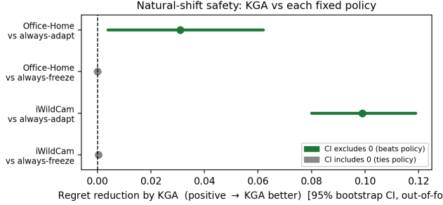
Fig. 5. Natural-shift safety at a glance. Regret reduction of KGA over each fixed policy (positive \rightarrow KGA better) with 95% bootstrap CIs under a valid out-of-fold radius. On both Office-Home and iWildCam, KGA beats always-adapt (CI excludes zero) and ties always-freeze (CI includes zero): no-harm / damage-prevention, not a beats-both.
