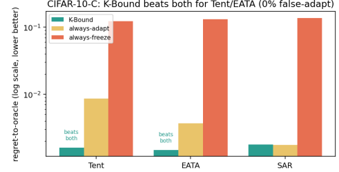
Fig. 10. CIFAR-10-C frontier (regret-to-oracle, log scale). KGA is below both always-adapt and always-freeze for Tent and EATA at 0% false-adapt, and ties always-adapt for SAR (Table XXVIII).
