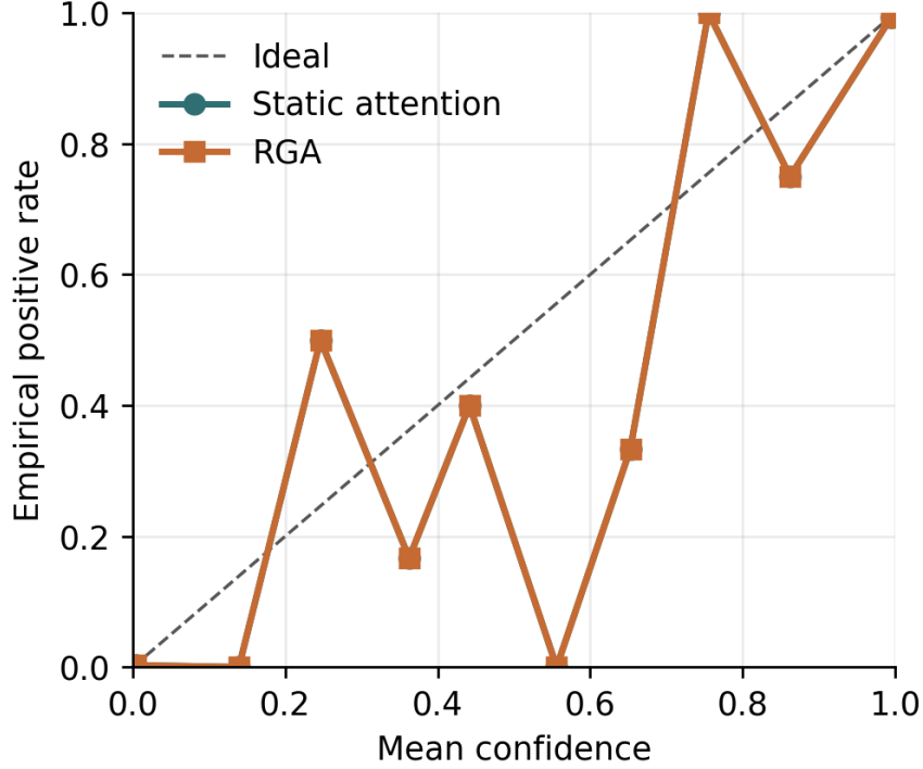
Figure 5: Reliability diagram for static attention and RGA.
