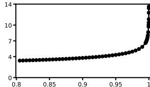
fashion_mnist
