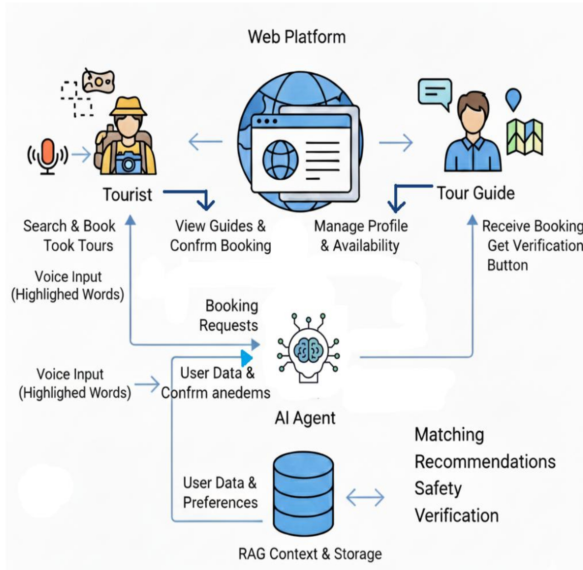
Figure 2: System High level Architecture Diagrams
