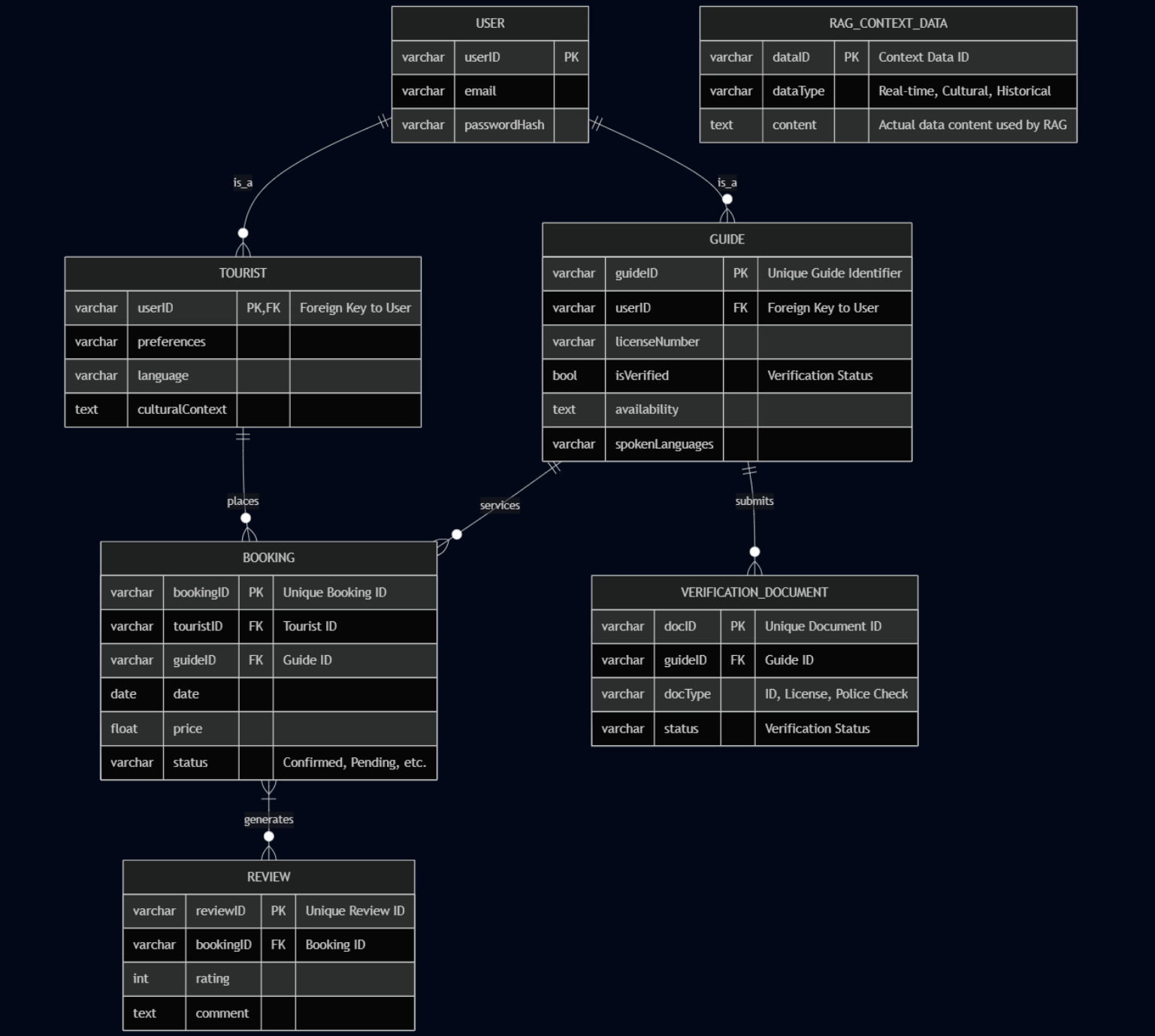
Figure 20 : Relationship Diagram
