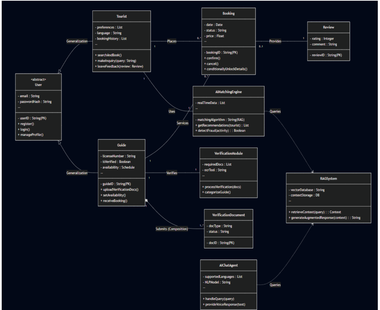
Figure 19 : Class Diagram
