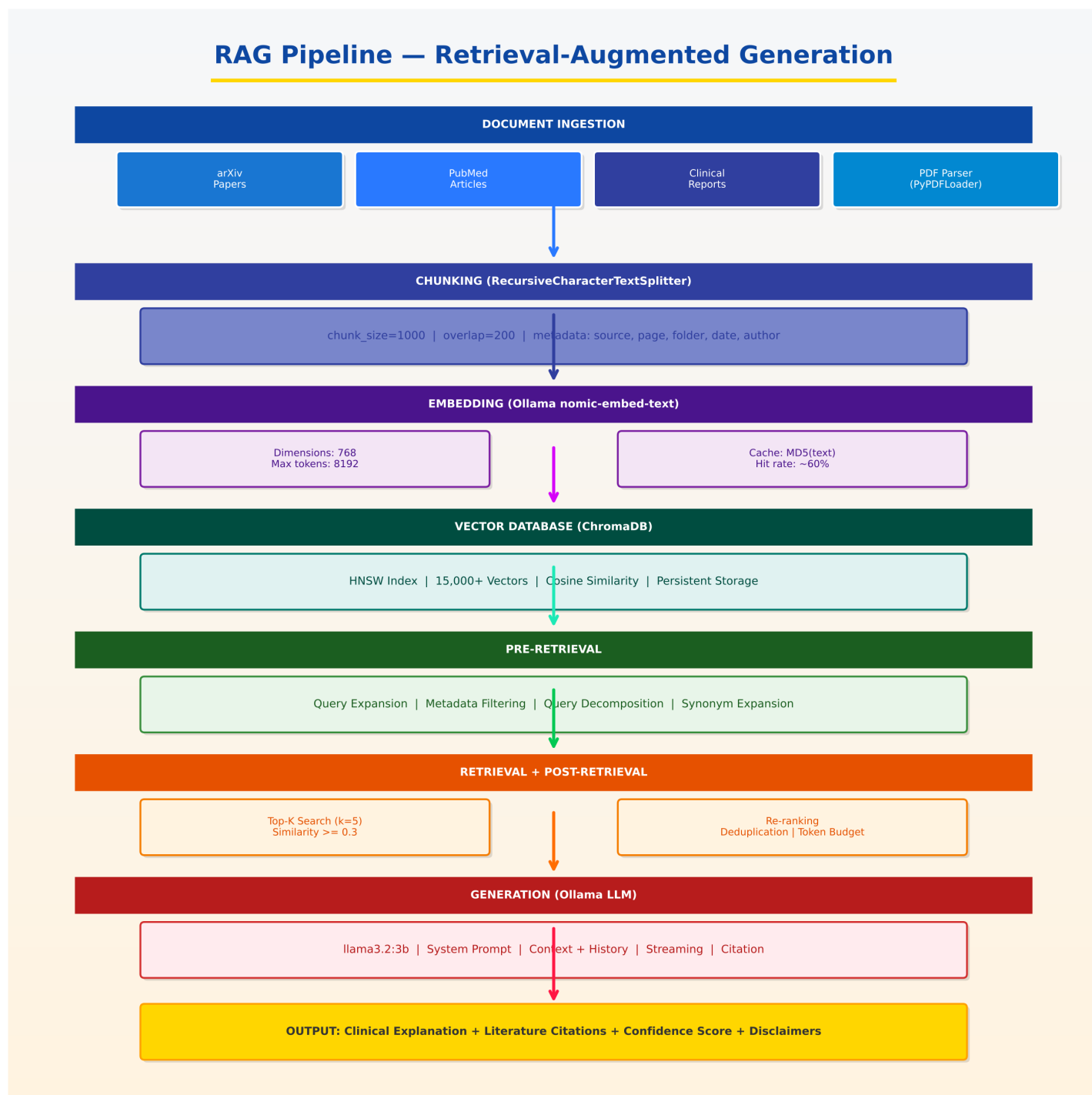
Figure 5: RAG Pipeline
