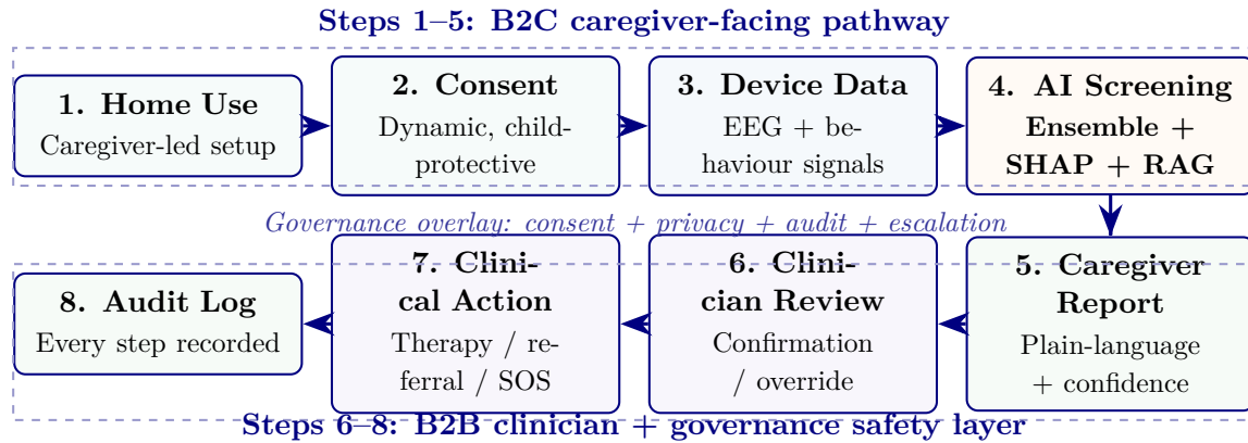
Figure 5.29. B2C-primary ASD screening pathway. Steps 1–5 are caregiver-facing (home setup, consent, device capture, AI screening, plain-language report). Steps 6–8 are the B2B safety layer (clinician review, clinical action, audit log). The dashed overlay indicates that consent, privacy, audit, and escalation governance apply continuously, not as a single checkpoint.
