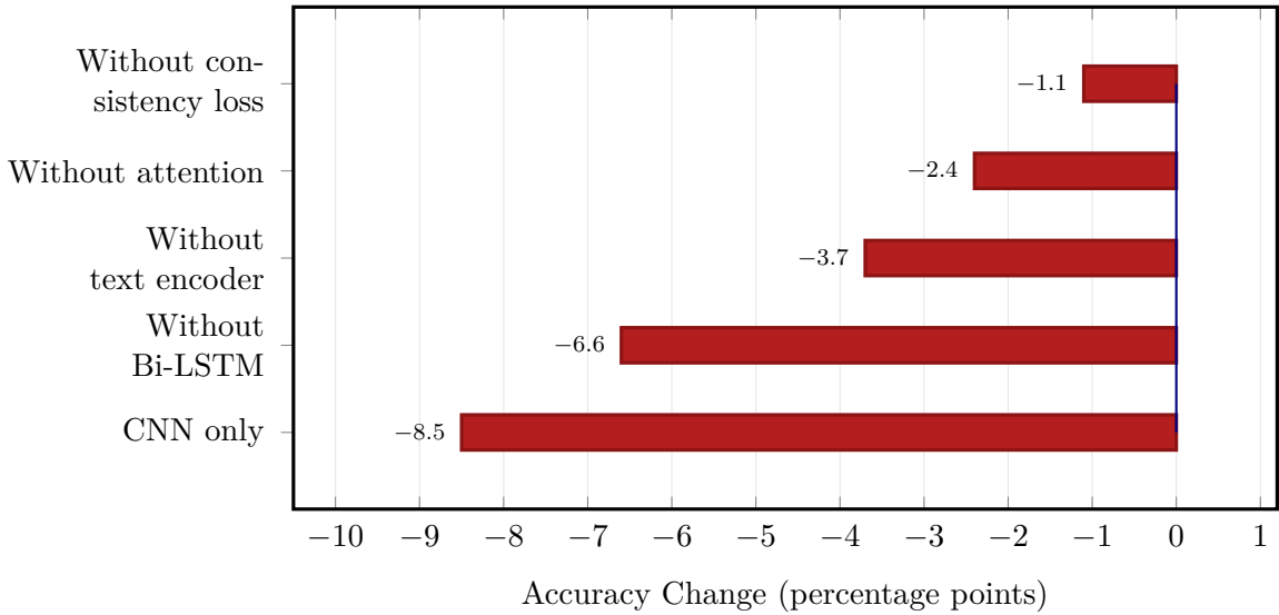
Figure 4.16. EEG-RAG VotingClassifier ablation: accuracy change when each component is removed from the full model (94.7% baseline). CNN-only baseline shows the largest degradation (−8.5 pp); Bi-LSTM removal costs −6.6 pp, confirming the importance of temporal modelling for EEG classification.
