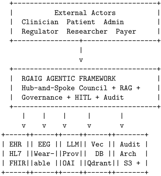
Figure 5.30. C4 Level 1 — System Context. The RGAIG framework as a single black-box system, with external actors (clinician, patient, administrator, regulator, researcher, payer) and external systems (EHR, wearable EEG, LLM provider, vector DB, audit archive). Internal structure is opened in Levels 2–4.
