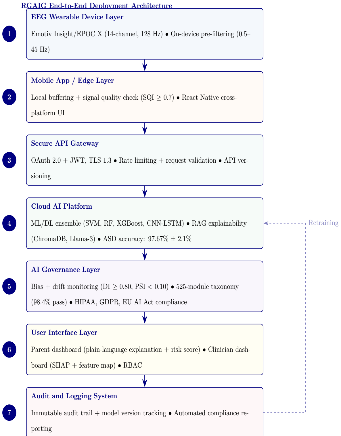
Figure 5.7. End-to-End Deployment Architecture. Seven-layer deployment stack from EEG wearable capture through cloud AI processing and governance to audit logging, with a retraining feedback loop from Layer 7 to Layer 4.
