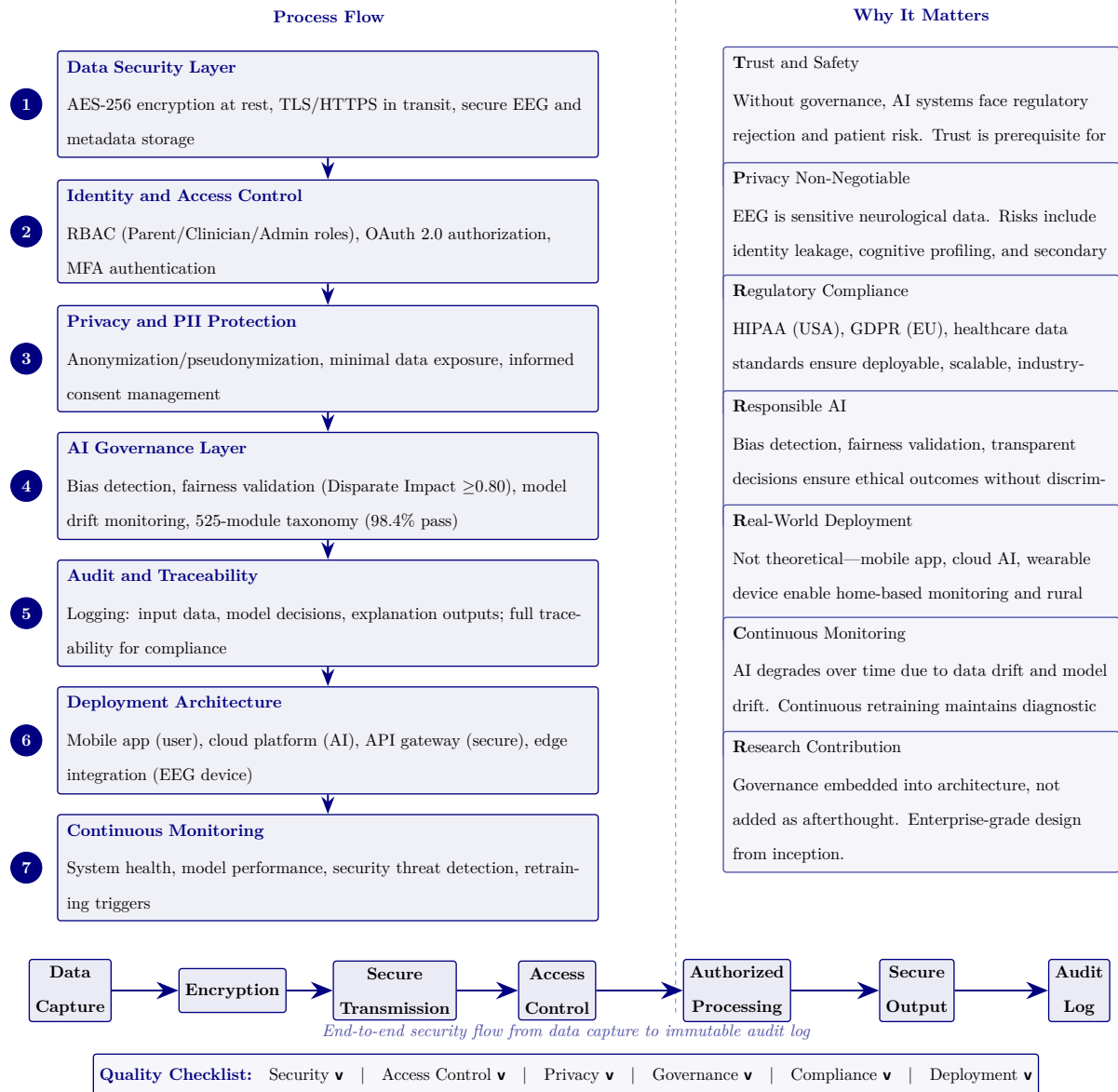
Figure 3.19. Phase 7: Governance, Security, Compliance, and Deployment Architecture
