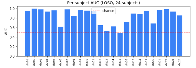
Fig. 4. Per-subject LOSO performance across the 24 CHB-MIT subjects.
