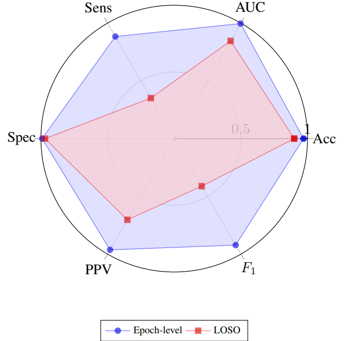
Fig. 1. Epoch-level vs LOSO across six metrics. Sensitivity is where the protocols diverge most.
