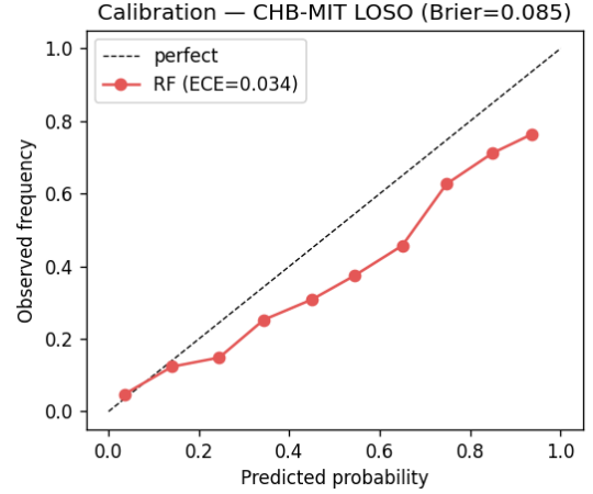
Fig. 3. Reliability (calibration) curve under CHB-MIT LOSO.
