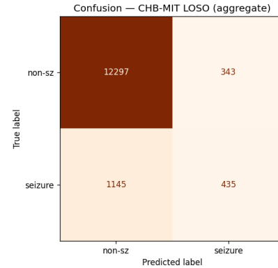
Fig. 5. CHB-MIT LOSO aggregate confusion matrix (pooled over 24 subjects).
