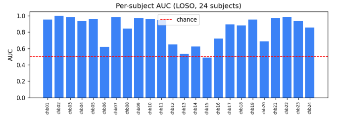
Fig. 3. Per-subject LOSO performance across the 24 CHB-MIT subjects.
