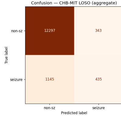
Fig. 4. CHB-MIT LOSO aggregate confusion matrix (pooled over 24 subjects).
