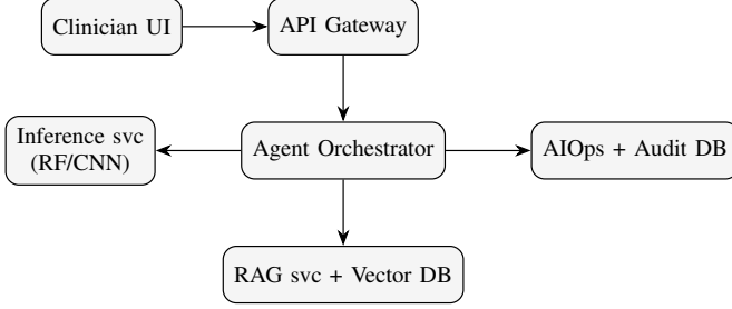
Fig. 7. Deployment network (C4 container view).
