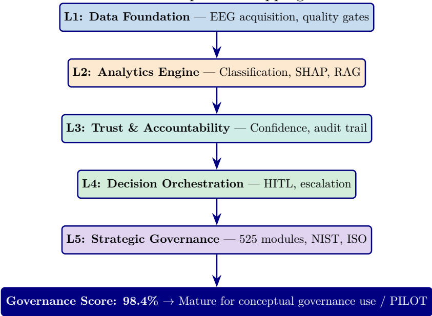
Figure 3.23. RGAIG Five-Layer Governance Framework. Each layer processes data from the layer above. The governance score (98.4%) determines the evaluation decision. 525 modules span 3 tiers: 8-phase ML/DL, 13-phase GenAI QA, 10 cross-cutting pillars.
