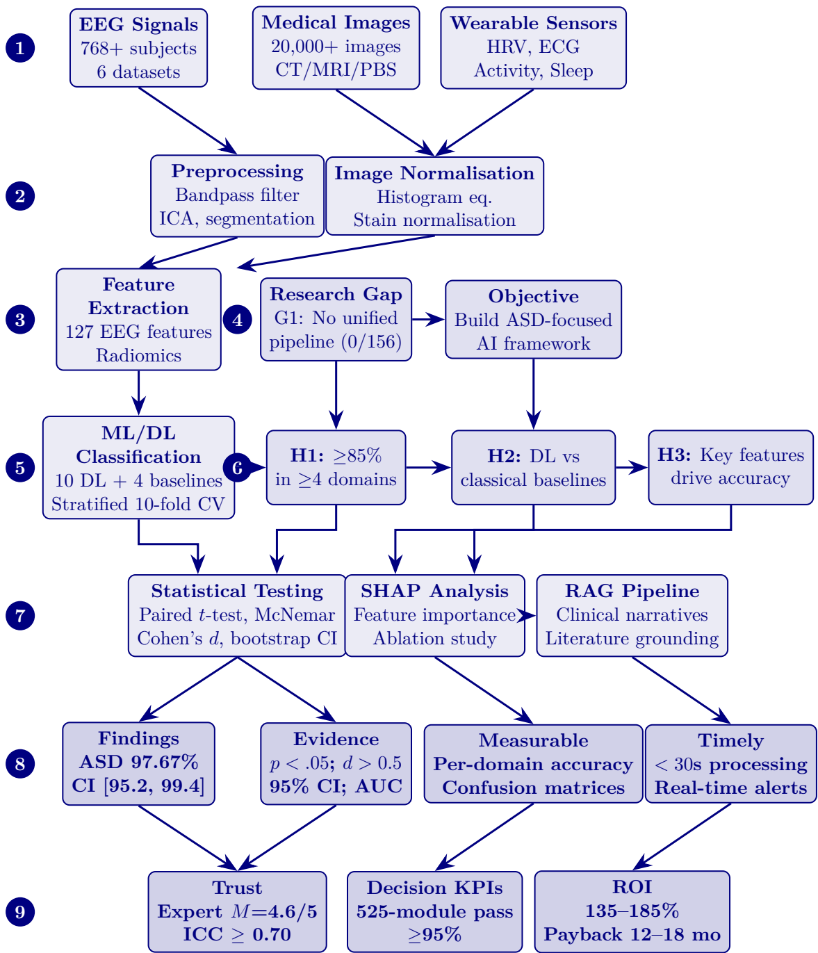
Figure 3.5. Pipeline 1 (9 steps): Secondary data quantitative analysis flow—from EEG/imaging/sensor data through preprocessing, feature extraction, ML/DL classification, and hypothesis testing to measurable findings with trust, decision KPIs, and illustrative financial scenario outcomes.
