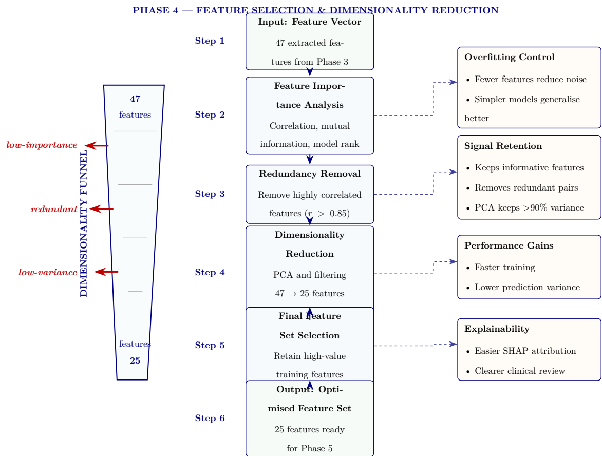
Figure 3.31. Phase 4: feature selection and dimensionality reduction. The 47 features from Phase 3 undergo importance ranking, redundancy removal, and PCA-based reduction to a 25-feature set that retains more than 90% of variance.
