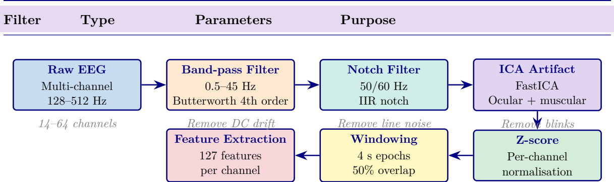
Figure 3.25. Seven-Stage EEG Signal Processing Pipeline from the EEG-RAG Framework
