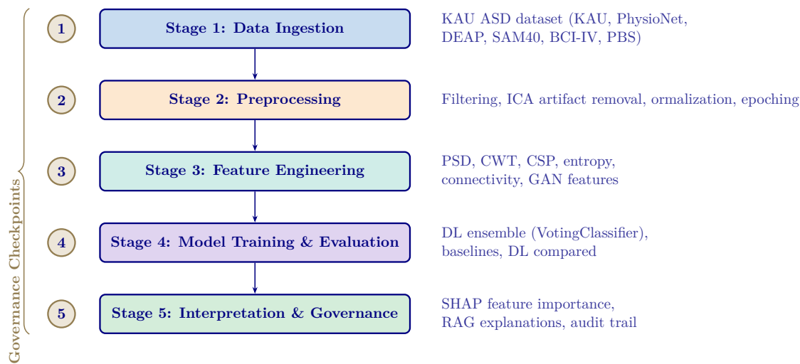
Figure 3.38. Five-Stage Analytical Pipeline for ASD Diagnosis
