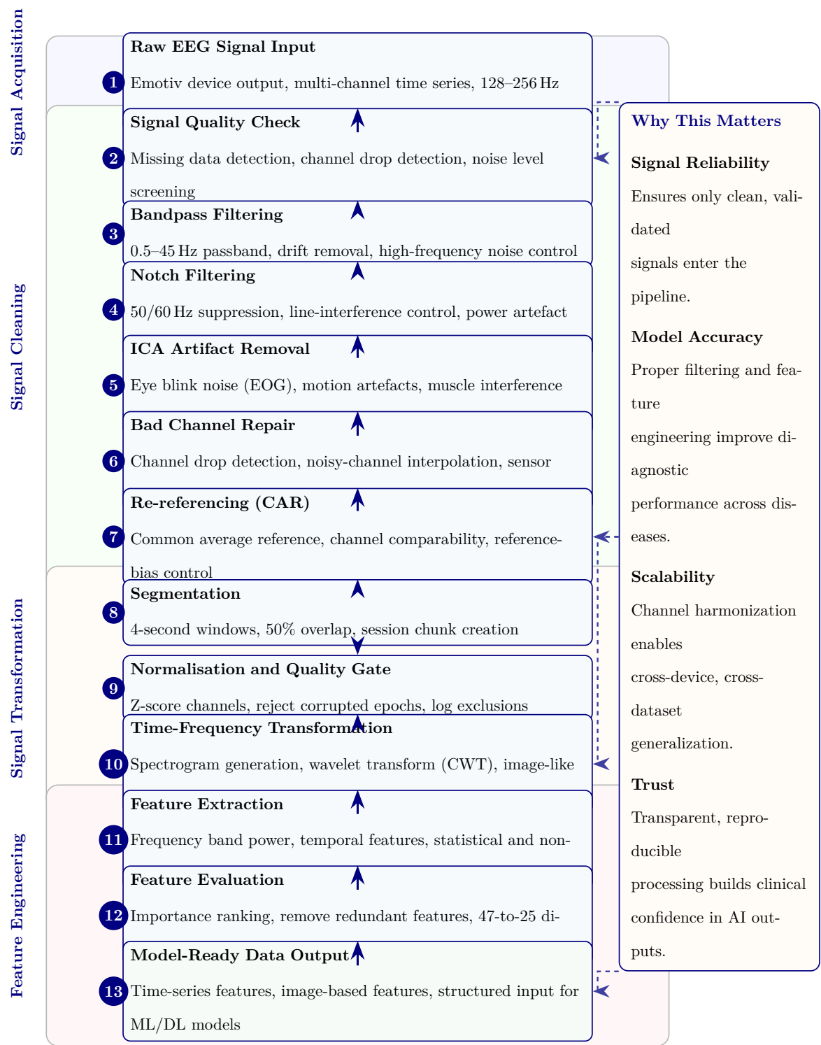
Figure 3.32. EEG Signal Processing Pipeline: From Raw Capture to Model-Ready Features
