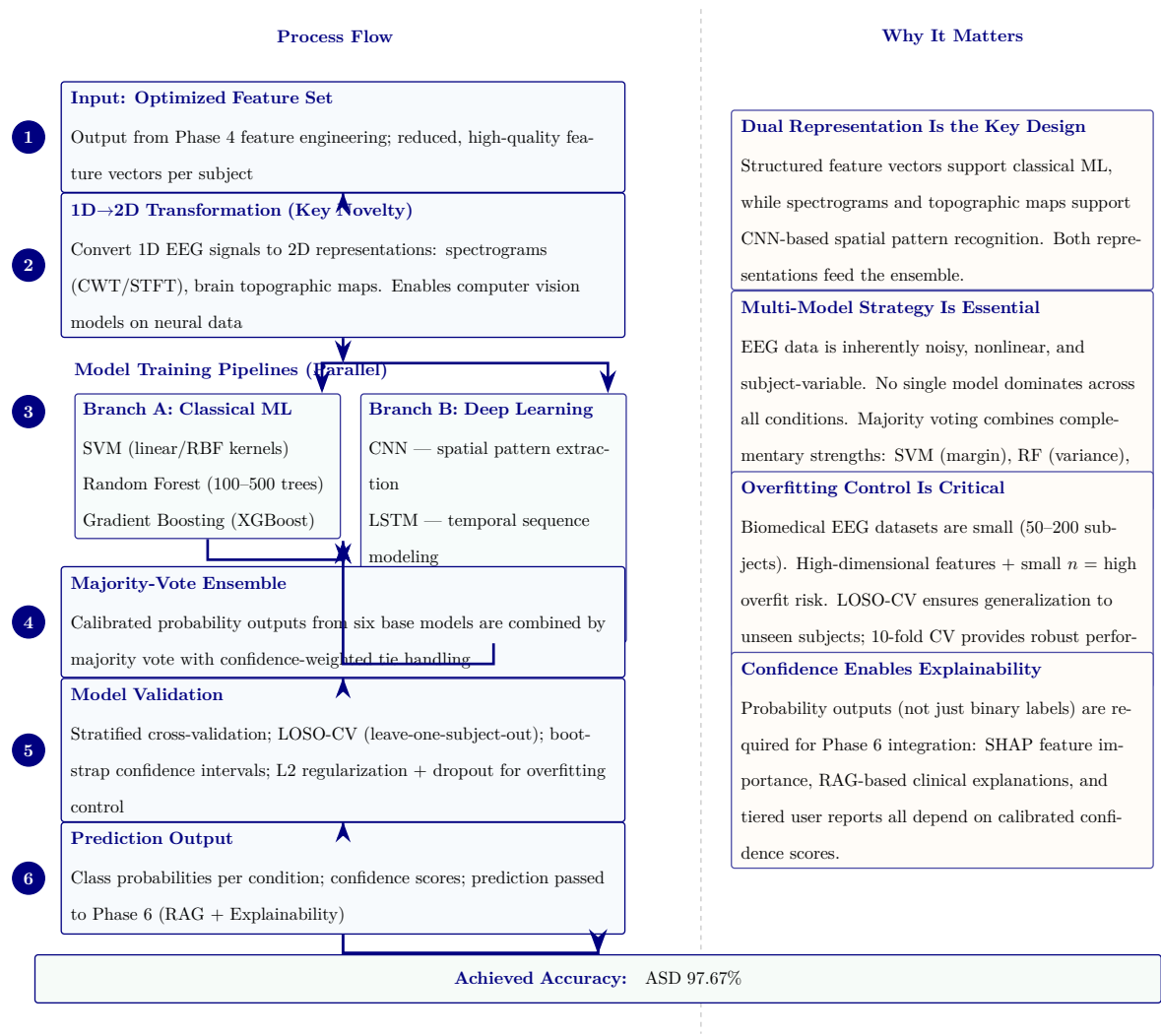
Figure 3.31. Phase 5: Hybrid AI model training and computer vision pipeline. The left column shows the six-step process from optimized features through 1D-to-2D transformation, parallel classical ML and deep learning pipelines, majority-vote ensembling, validation, and prediction output. The right column provides methodological justification for each design decision. Bottom row reports the achieved ASD classification accuracy (97.67%).
