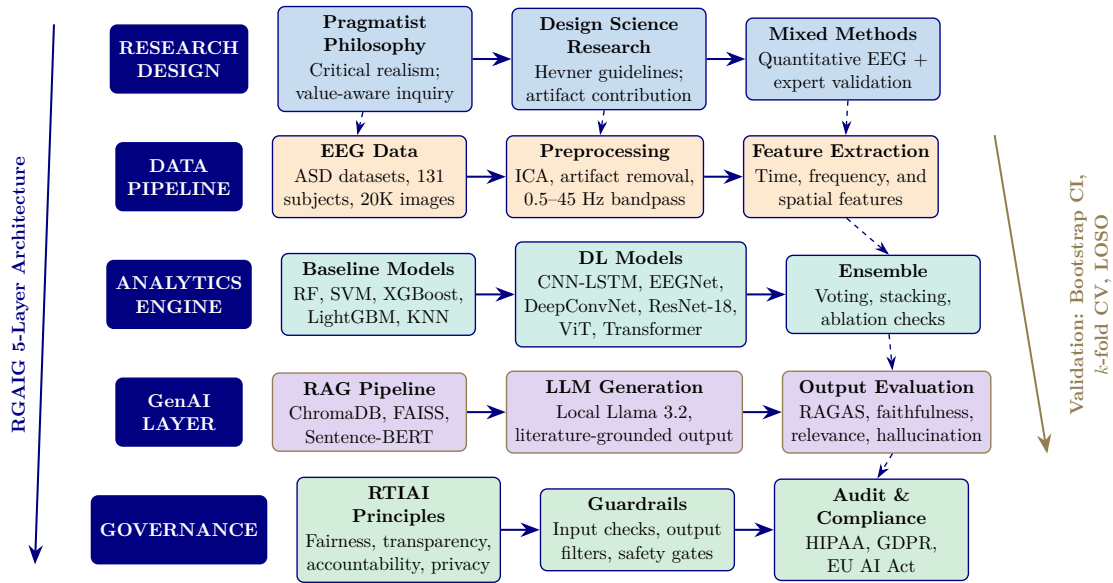
Figure 3.11. End-to-end methodology pipeline: research design, EEG data, analytics, generative AI, and governance mapped to the RGAIG five-layer architecture.
