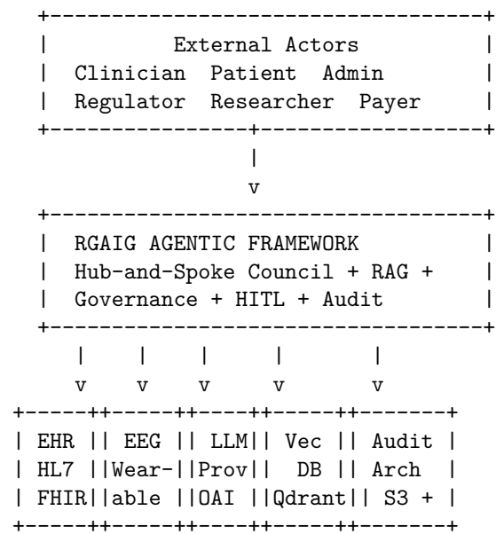
Figure 5.30. C4 Level 1 — System Context. The RGAIG framework as a single black-box system, with external actors (clinician, patient, administrator, regulator, researcher, payer) and external systems (EHR, wearable EEG, LLM provider, vector DB, audit archive). Internal structure is opened in Levels 2–4.
