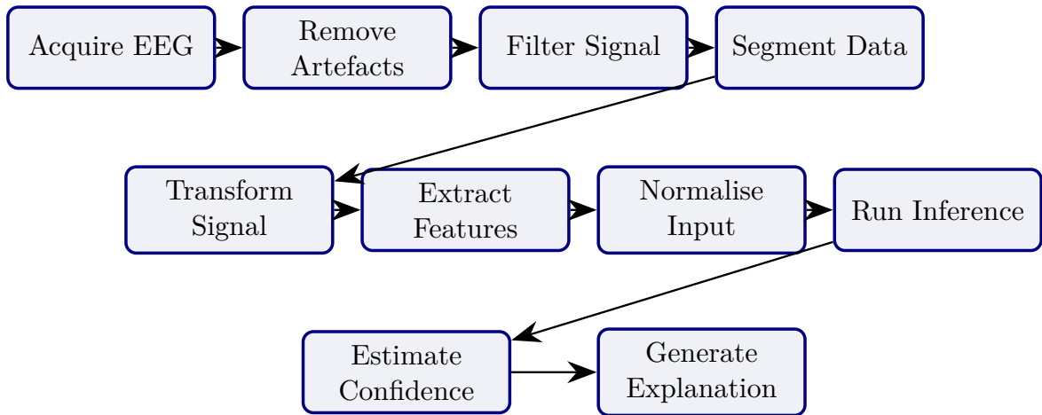
Figure 3.36. Secondary EEG Processing Pipeline
