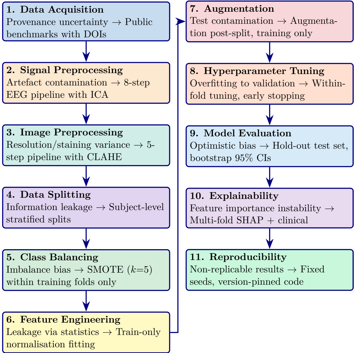
Figure 3.12. End-to-End Data Defence Summary: Pipeline Stages, Threats, and Safeguards
