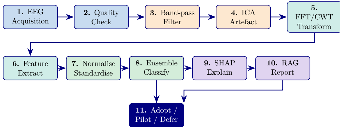
Figure 3.3. Part B: 11-Stage EEG Analysis Pipeline Flowchart. Stages 1–5 (blue/orange) cover data acquisition and preprocessing; Stages 6–7 (teal/green) cover feature engineering and normalisation; Stages 8–10 (green/purple) cover classification, explainability, and reporting; Stage 11 (navy) delivers the evaluation decision.
