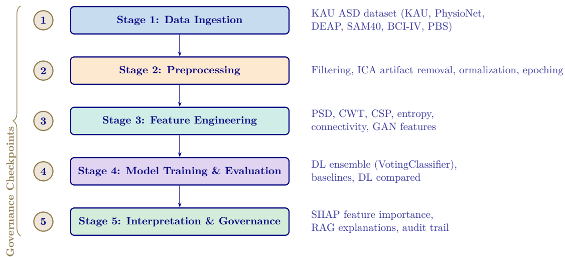
Figure 3.37. Five-Stage Analytical Pipeline for ASD Diagnosis
