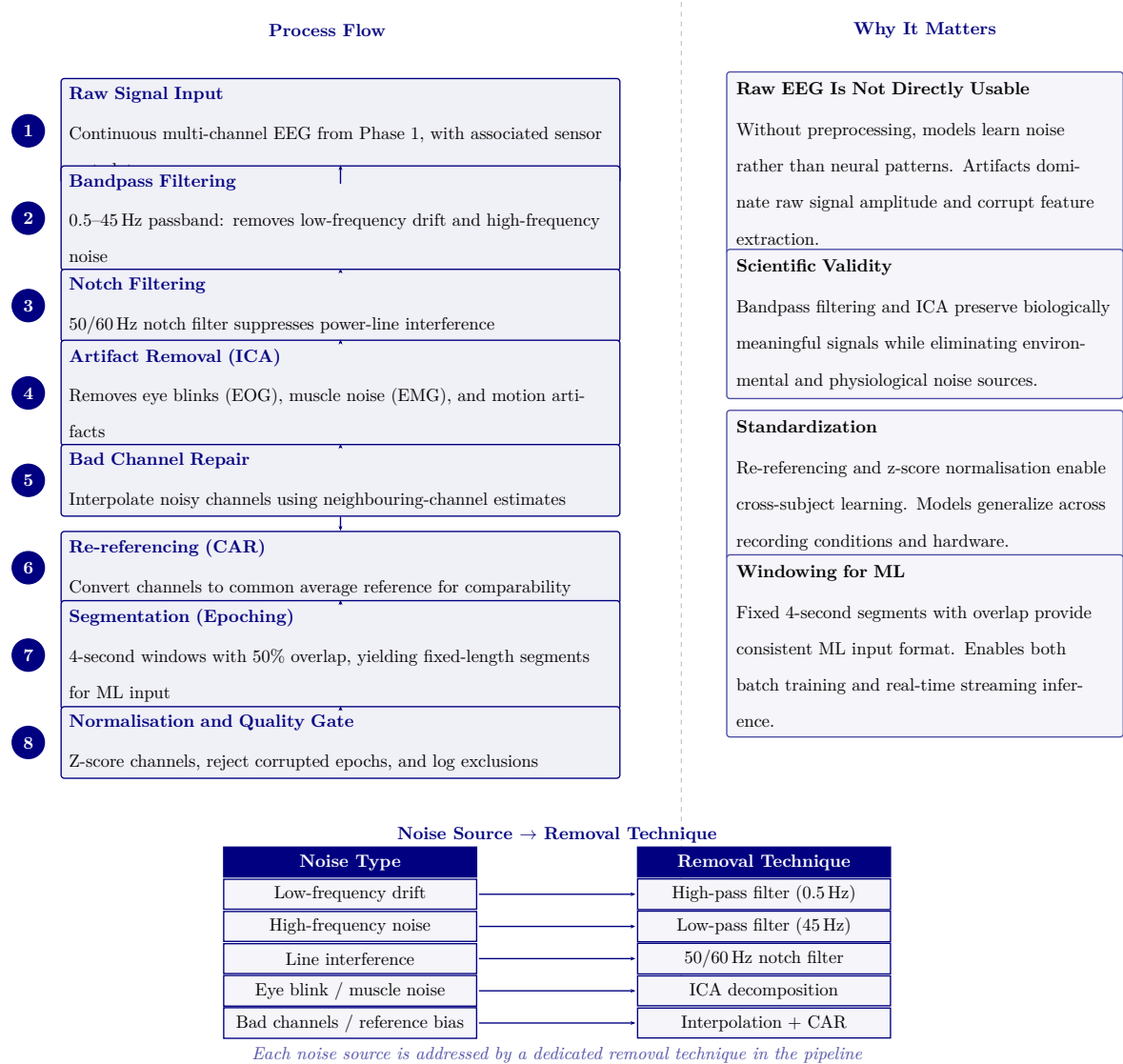
Figure 3.28. Phase 2: Signal Preprocessing and Cleaning Pipeline
