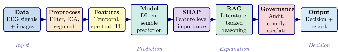
Figure 3.9. End-to-end RGAIG pipeline: data flows through preprocessing, feature engineering, DL prediction, dual explainability (SHAP + RAG), governance validation, and decision output.
