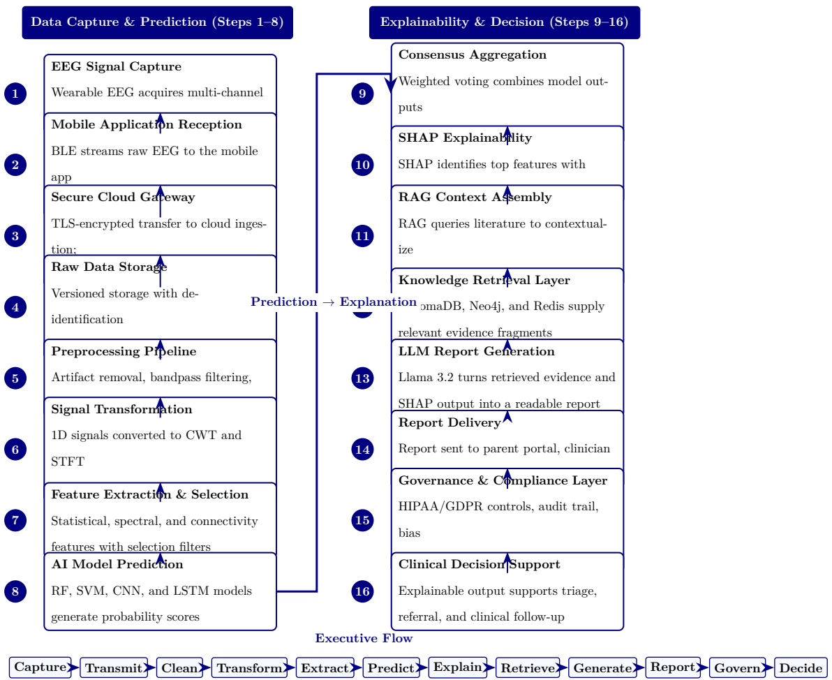
Figure 3.34. RGAIG end-to-end data flow: 16-stage pipeline from EEG capture to clinical decision support.
