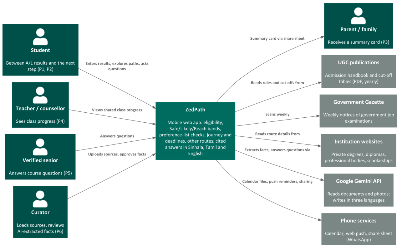
Figure 1: ZedPath system context (C4 model, level 1)
