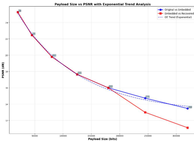
Fig. 7. PSNR vs Payload size along with embedded vs recovered
