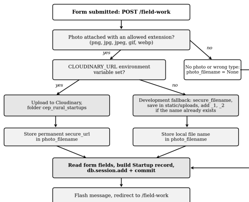
Figure 5.3: Photo upload workflow of the Field Work form.
