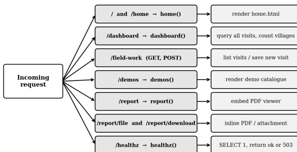
Figure 5.2: Routing map of the website.
