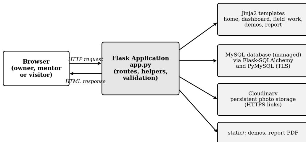
Figure 5.1: Architecture of the project website.
