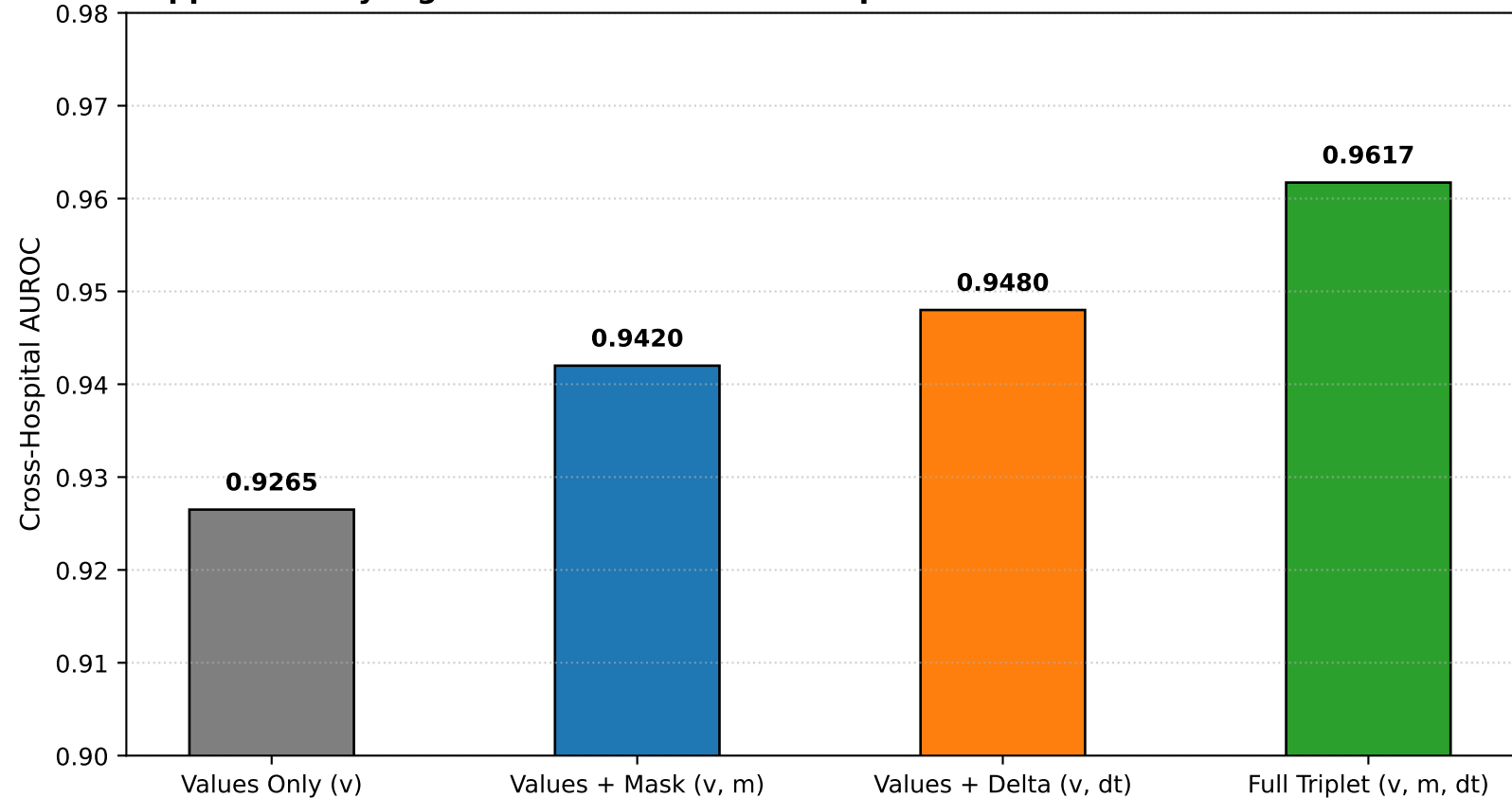
Supplementary Figure S1: 2x2 Factorial Component Ablation Main Effects
