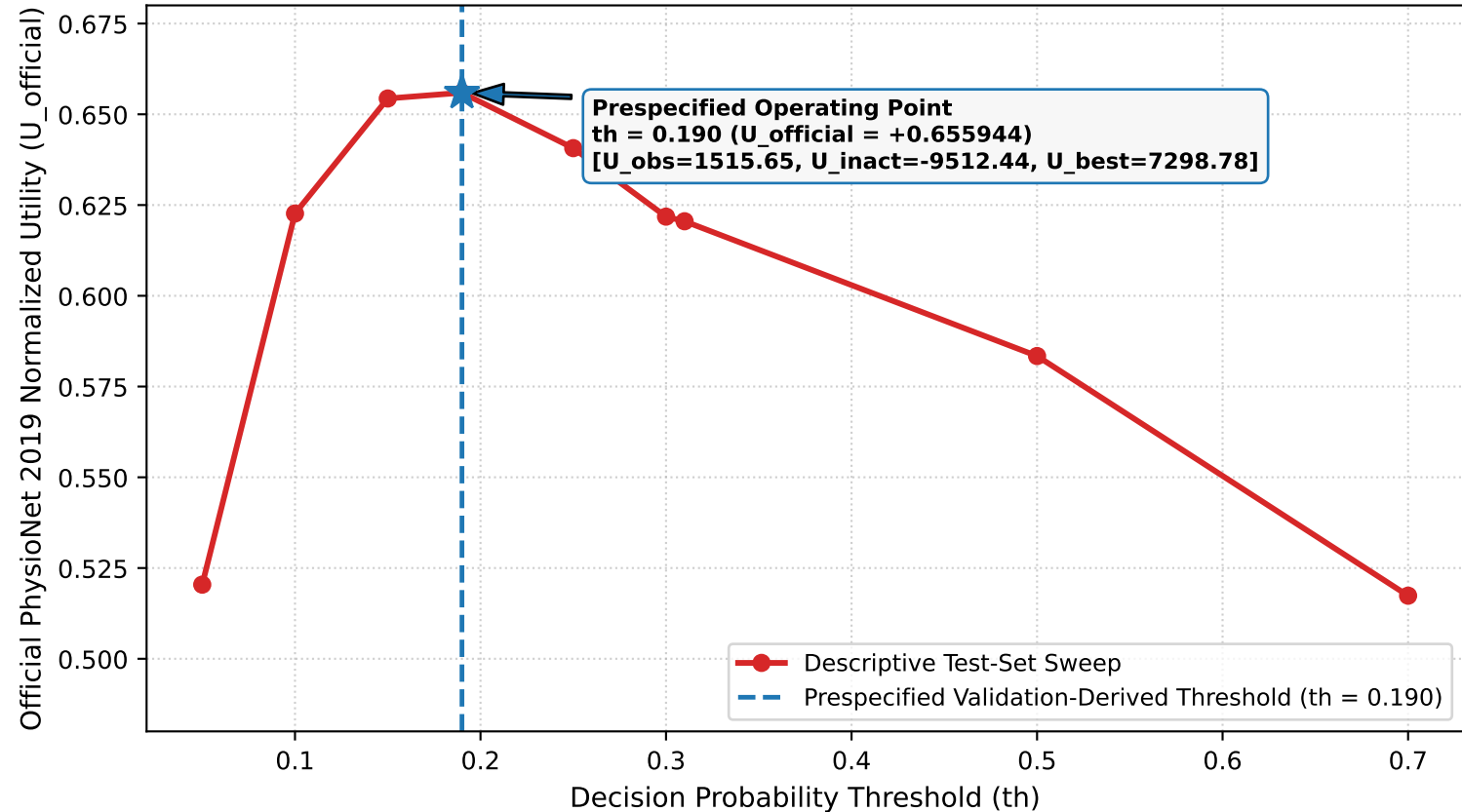
Figure 4. Official PhysioNet utility across decision thresholds.
