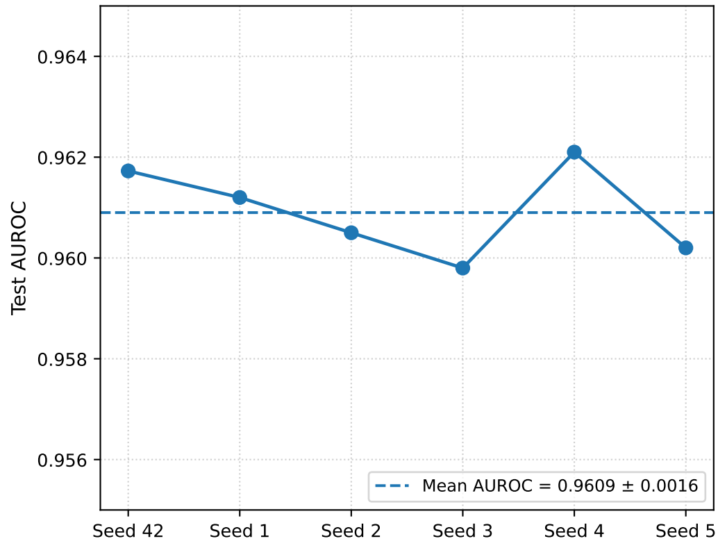
A: Random Initialization Stability (6 Seeds)
