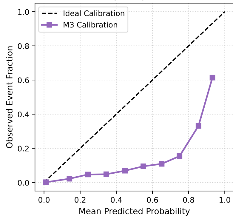
A: M3 Reliability Diagram
