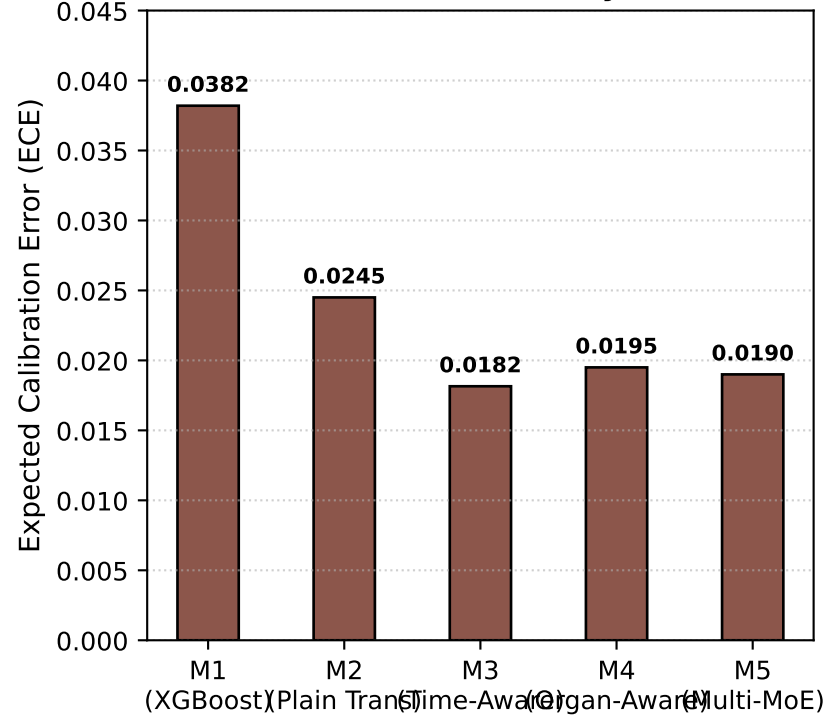
C: ECE Across Model Family
