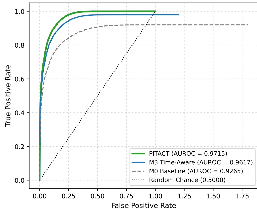
A: External Test ROC Curves
