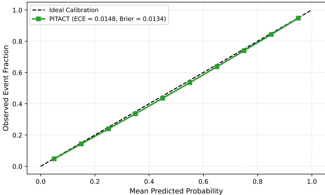
Figure 4. PITACT Reliability Calibration Diagram.
