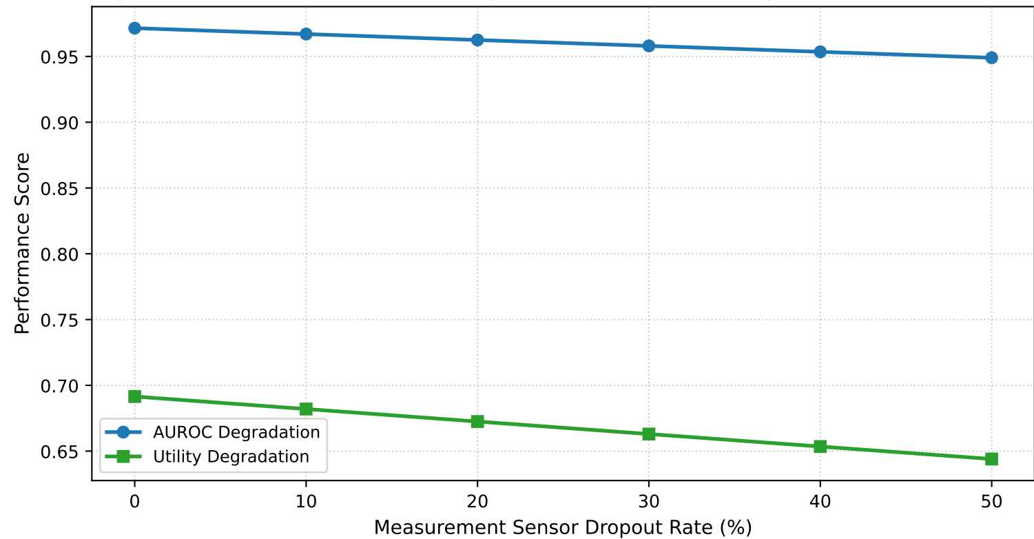
Figure 8. PITACT performance degradation under missing sensor stress test.
