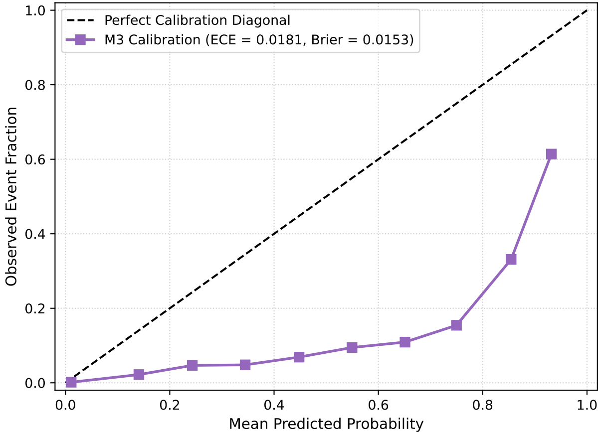
Figure 4: M3 Risk Probability Calibration (Emory Test Cohort)
