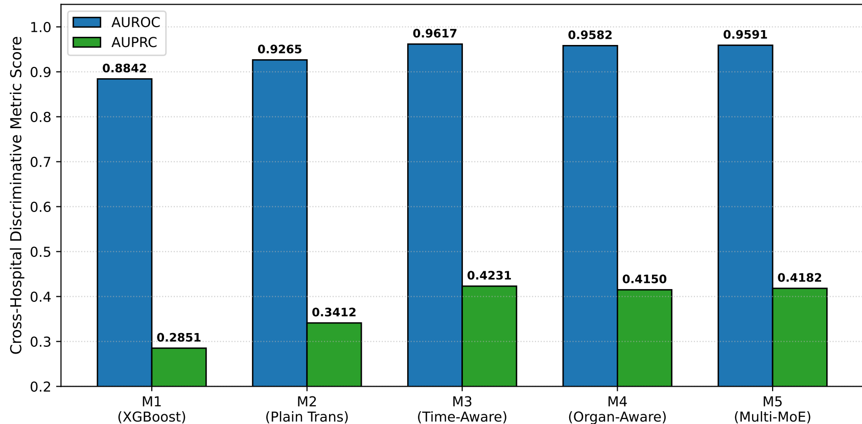
Figure 7: Model Family Discriminative Performance (Emory Test Set)
