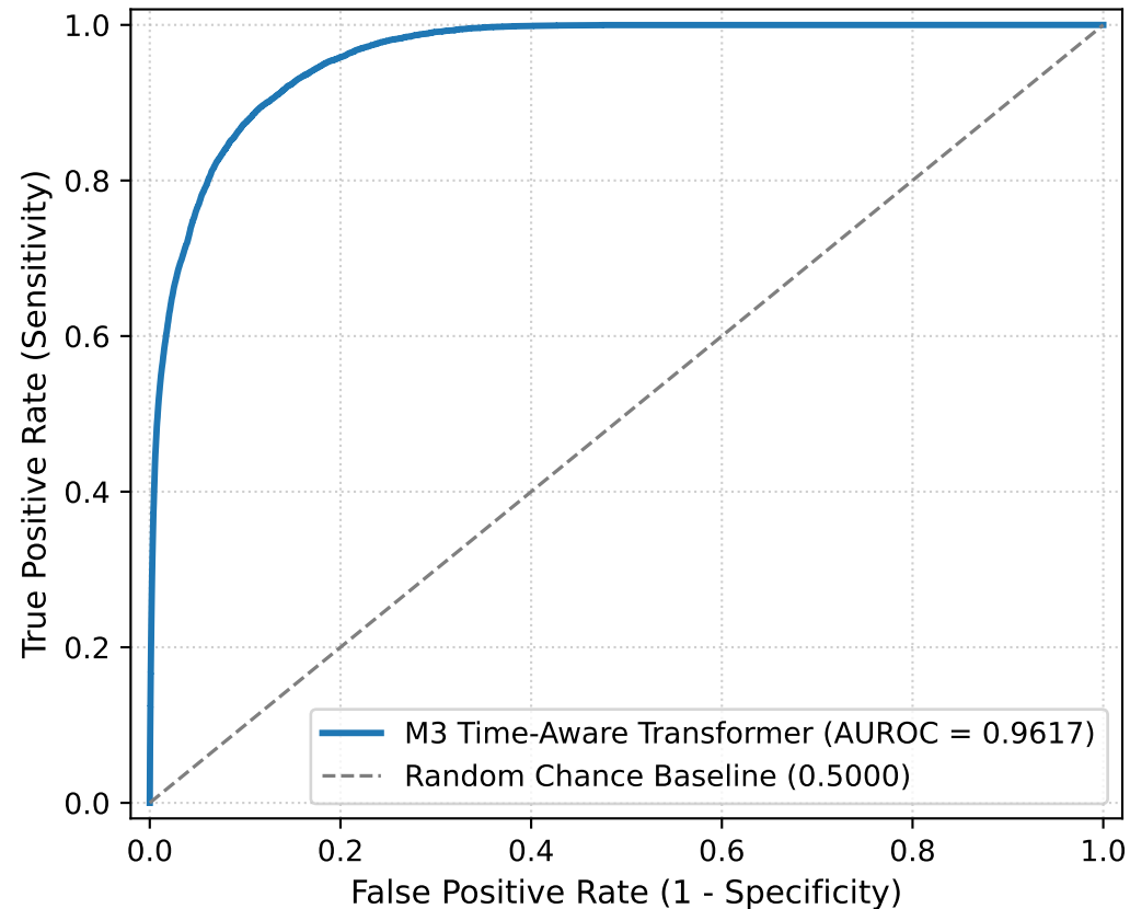
A: Receiver Operating Characteristic (ROC)
