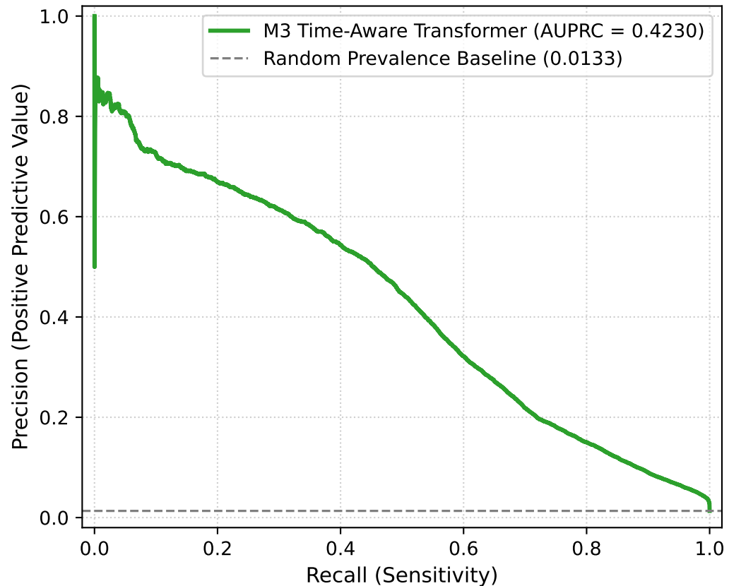
B: Precision-Recall (PR) Curve
