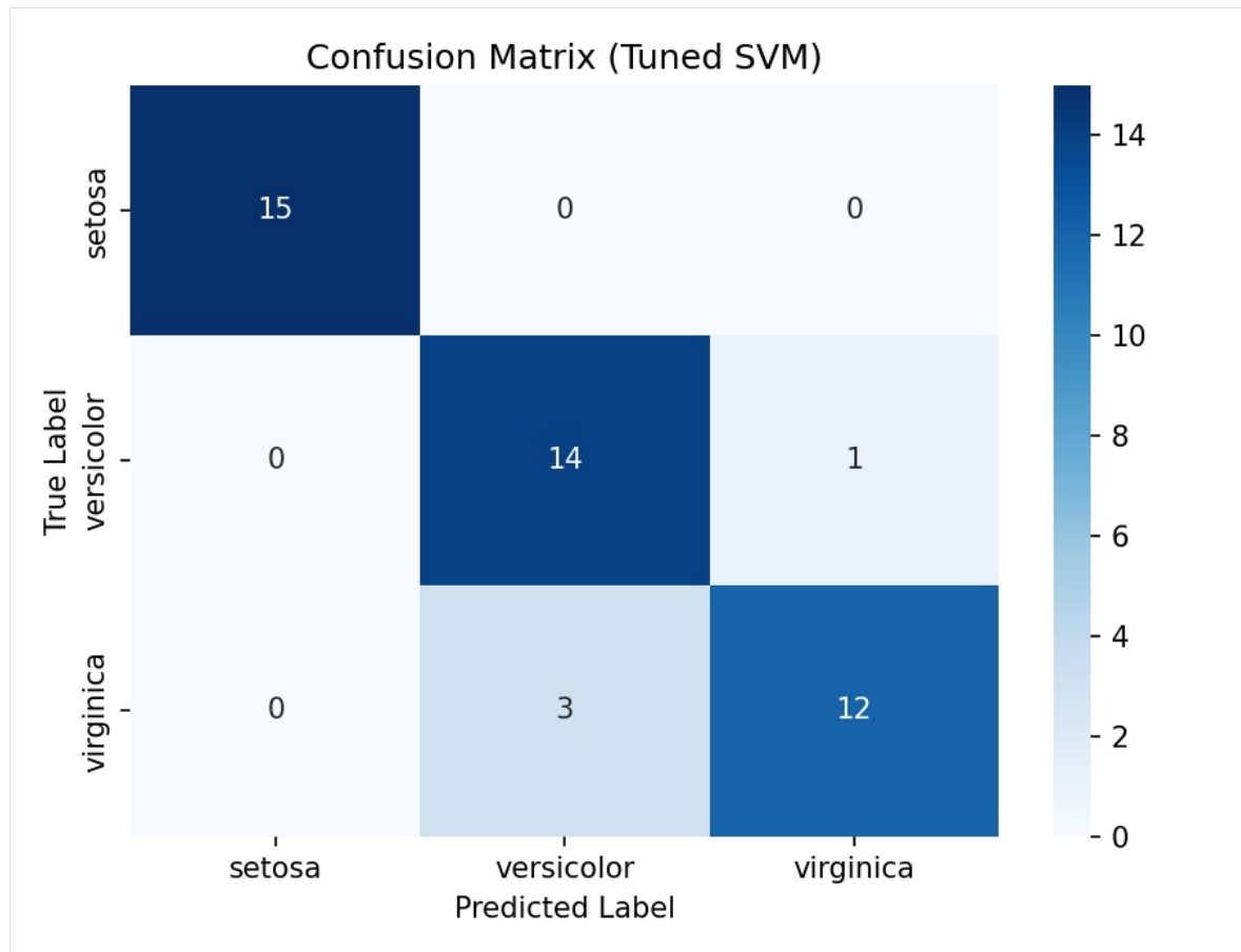
Fig 1. Confusion Matrix (Tuned SVM)
