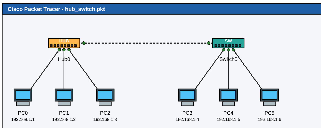
Experiment 3 : hub and switch in the same network
