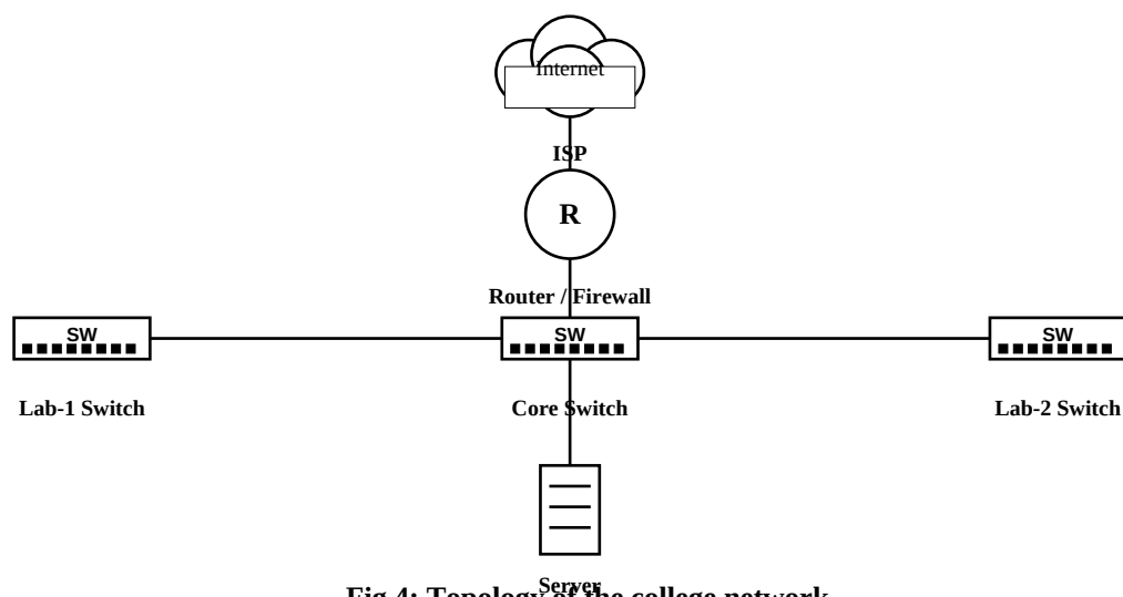
Fig 4: Topology of the college network
