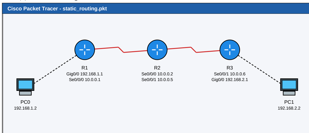
Packet Tracer view (red lightning lines are serial links)
