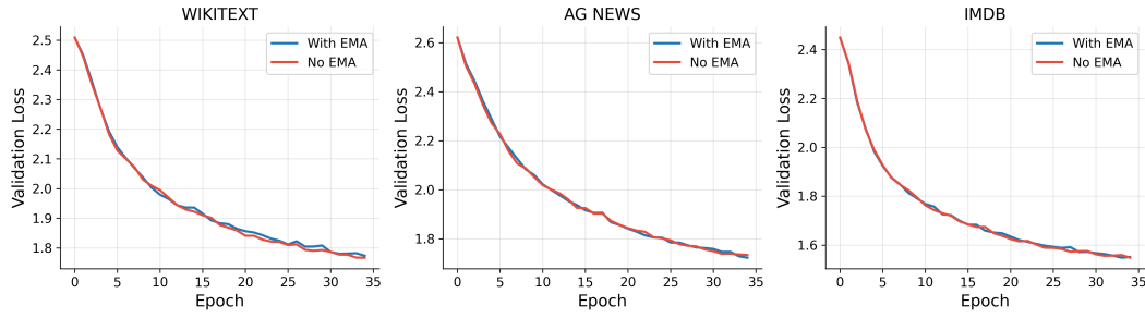
Figure 8: Comparison of sample statistic tracking with and without EMA across all datasets.
