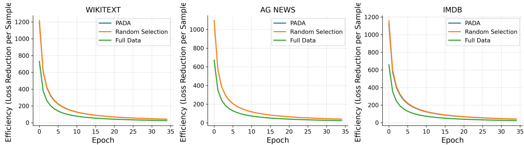
Figure 10: Training efficiency (validation loss reduction per sample) over epochs for all datasets.
