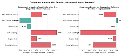
Figure 3: Component contribution analysis showing average metric changes when removing each component. Early stopping removal causes largest degradation (+0.23 TCE, -0.13 ARR), followed by modality selector (+0.18 TCE, -0.09 ARR). Multi-dataset training shows beneficial effects (-0.10 TCE).
