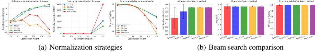
Figure 3: Decoding strategy ablations. (a) Normalization strategy critically affects perplexity: raw scores cause catastrophic degradation (reaching 10,000), while z-score and softmax maintain better fluency but still degrade structural validity to 0.81–0.82 at high weights. (b) Beam search improves adherence from 1.1 (sampling) to 1.8 (beam k \geq 3 ) with minimal fluency cost, but all methods achieve near-perfect structural validity regardless of search strategy, suggesting beam search mitigates some instability issues.
