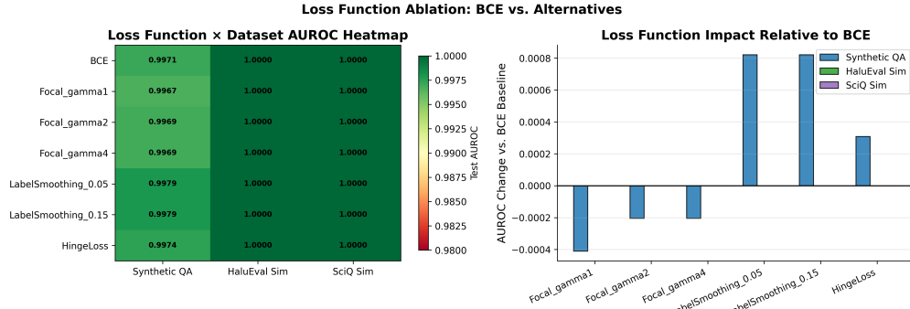
Figure 8: Loss function impact relative to BCE baseline (right) and absolute AUROC heatmap (left). Label smoothing (0.05) provides marginal gains on Synthetic QA (+0.0008); focal loss variants show small negative effects. All differences are \leq 0.0008 AUROC, confirming that loss function choice is essentially irrelevant in this near-ceiling performance regime.
