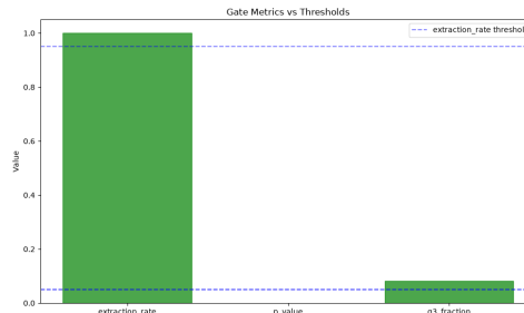
Figure 1: Gate validation metrics showing extraction rate (1.0), correlation p-value (NaN), and Q3 population (0.082) compared to thresholds. Two of three gates passed.
