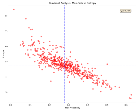
Figure 4: Quadrant analysis plot showing max-probability (x-axis) vs. entropy (y-axis). Q3 quadrant (upper-right, high max-prob and high entropy) contains 8.20% of predictions (41/500), all incorrect.
