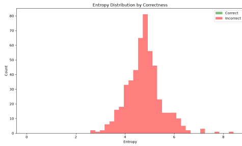
Figure 3: Overlaid histograms of entropy distributions for correct vs. incorrect predictions. Only the incorrect distribution exists (red), as GPT-2 achieved 0% accuracy.
