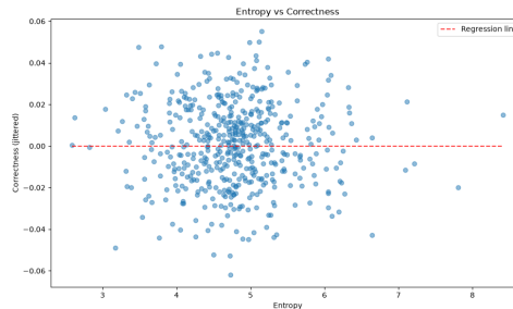
Figure 2: Scatter plot of entropy vs. correctness with binary jitter. All predictions lie on y=0 line (incorrect), demonstrating zero variance in correctness.
