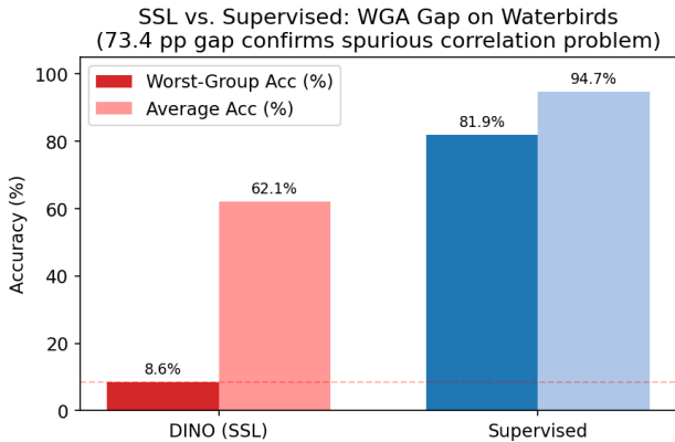
Figure 1. Figure 1: WGA and average accuracy comparison — DINO SSL vs. Supervised on Waterbirds.
