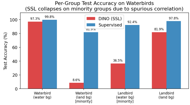
Figure 3. Figure 3: Per-group test accuracy for DINO SSL and supervised training on Waterbirds.
