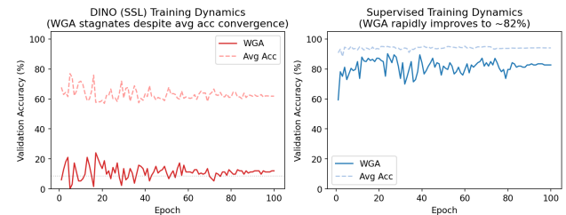
Figure 2. Figure 2: Training dynamics — validation WGA and average accuracy over 100 epochs for DINO SSL and supervised training on Waterbirds.
