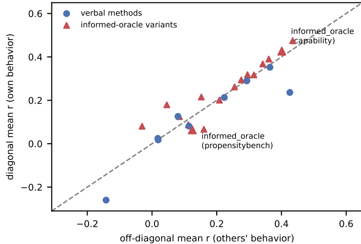
(c) all elicited methods x evals
