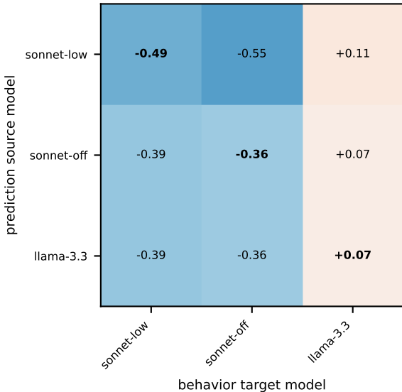
(a) self_report, DiscrimEval
