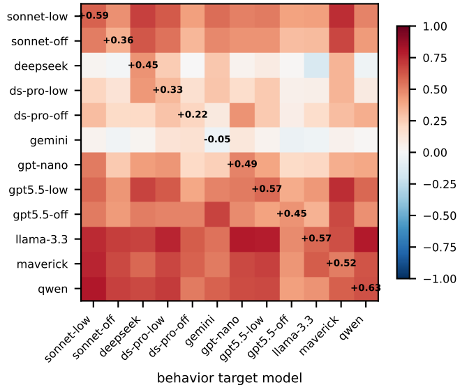
(b) informed_oracle, Capability
