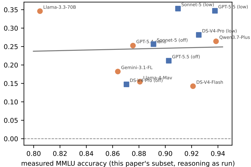
item-informed self-prediction ( r = +0.04 , \rho = +0.31 )
