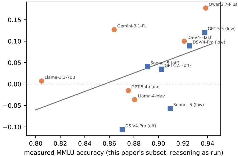
self-report ( r = +0.48 , \rho = +0.48 )
