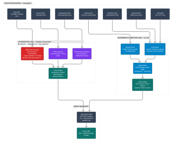
Figure 2. Ingestion architecture comparing deterministic parsing for schema/code with optional LLM-assisted extraction for requirements, policies, and RBAC documents.
