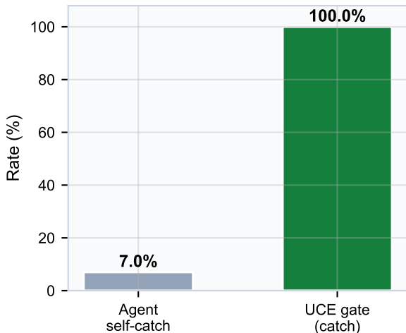
(a) Enforcement (114 scenarios, 4 repos)
