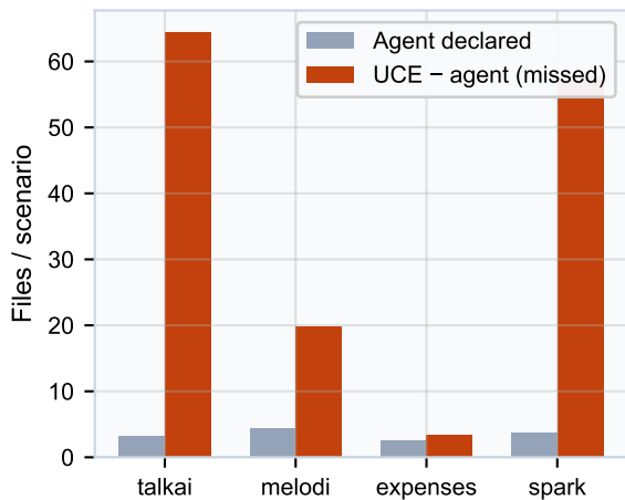
(c) Under-declaration by repository
