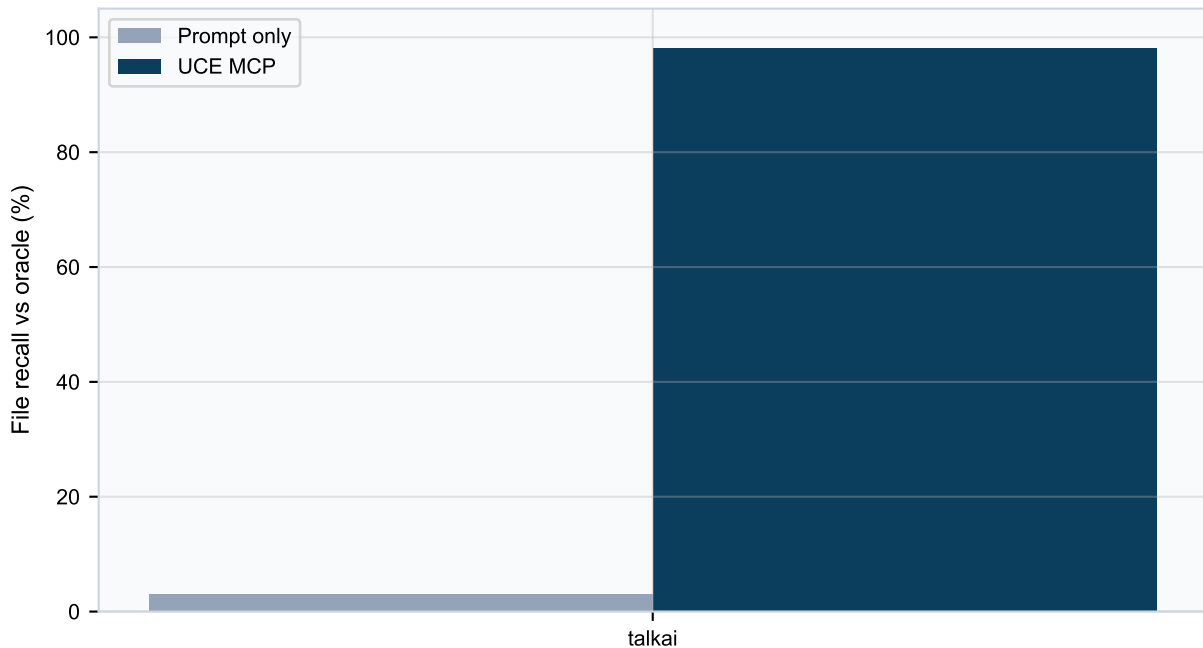
External validity: agent+MCP across repositories
