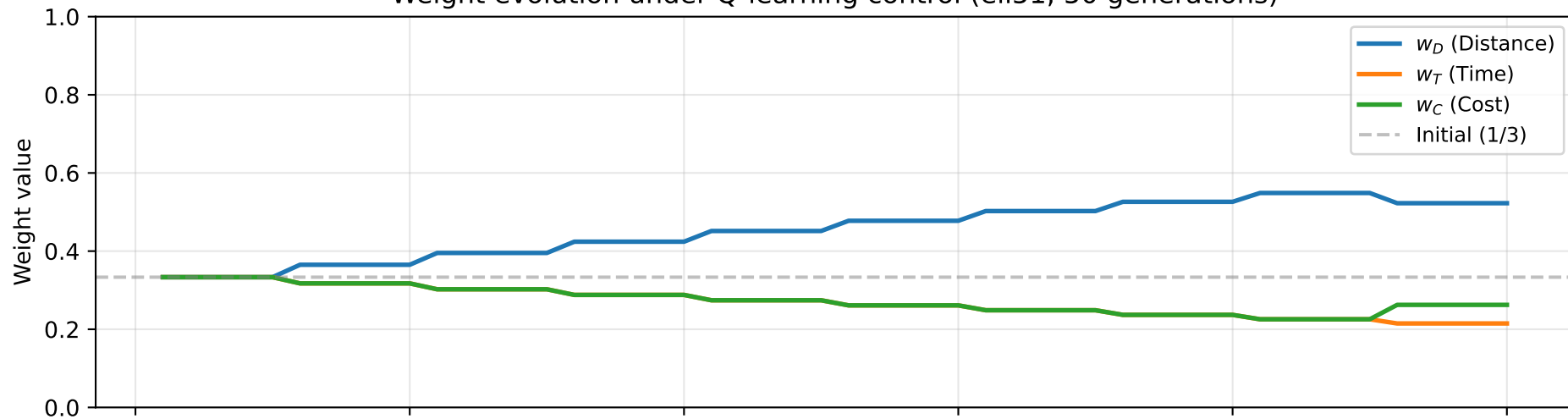
Weight evolution under Q-learning control (eil51, 50 generations)
