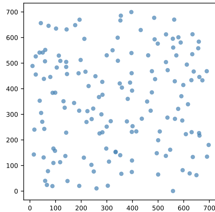
ch150 (150 cities)
