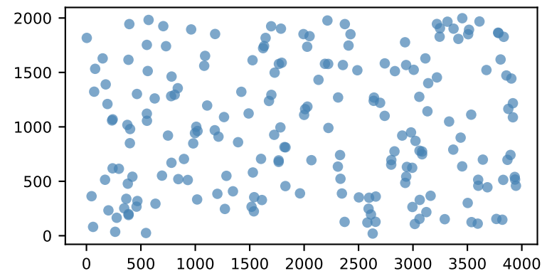
kroB200 (200 cities)
