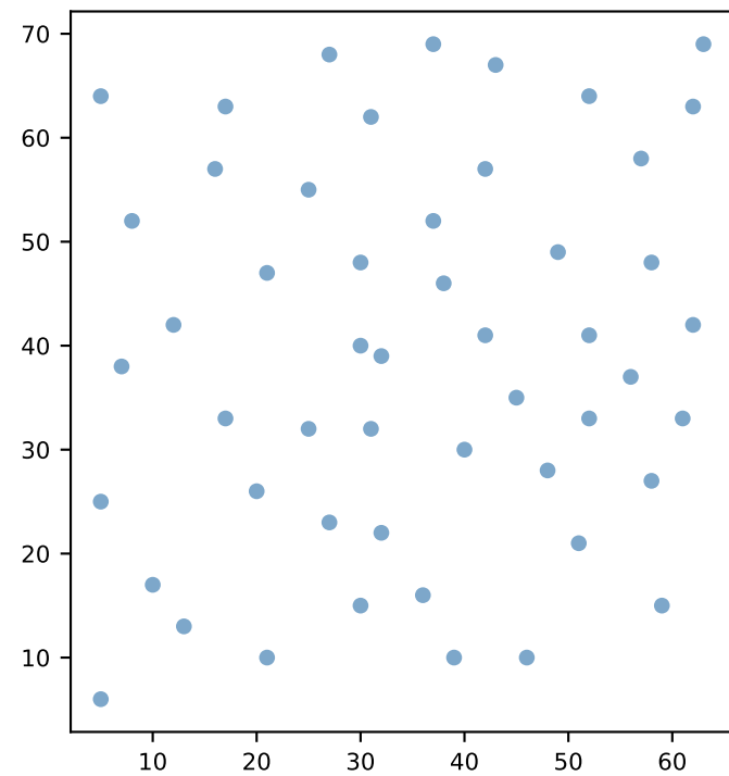
eil51 (51 cities)
