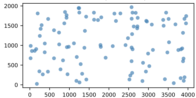
kroA100 (100 cities)
