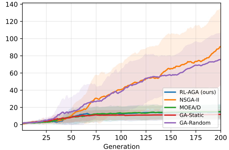
ch150
