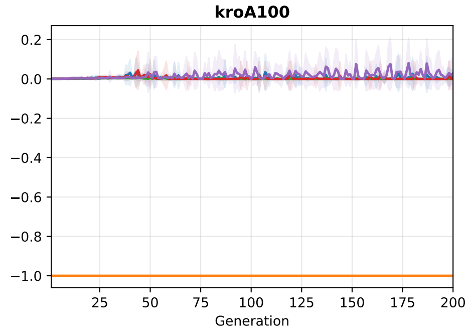
Convergence Curves — Mean \pm Std across 20 runs
