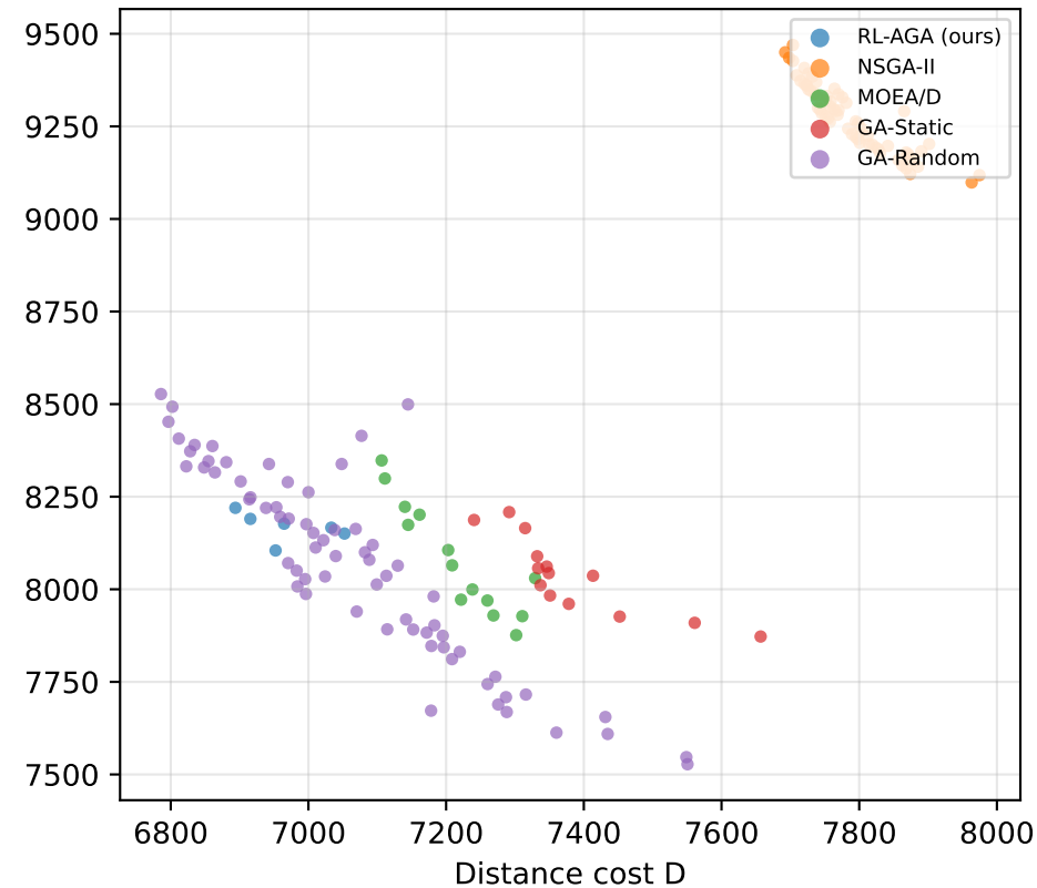
ch150
