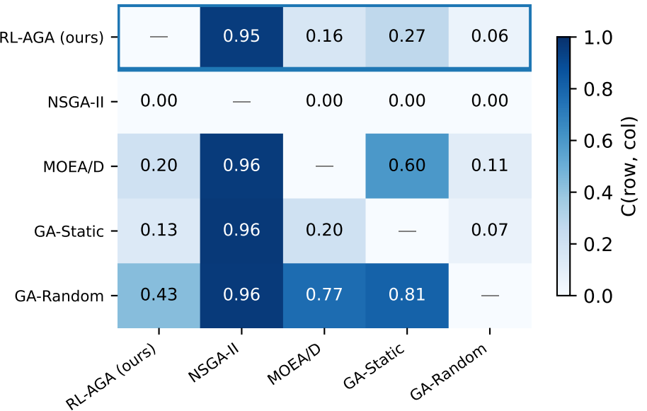
ch150
